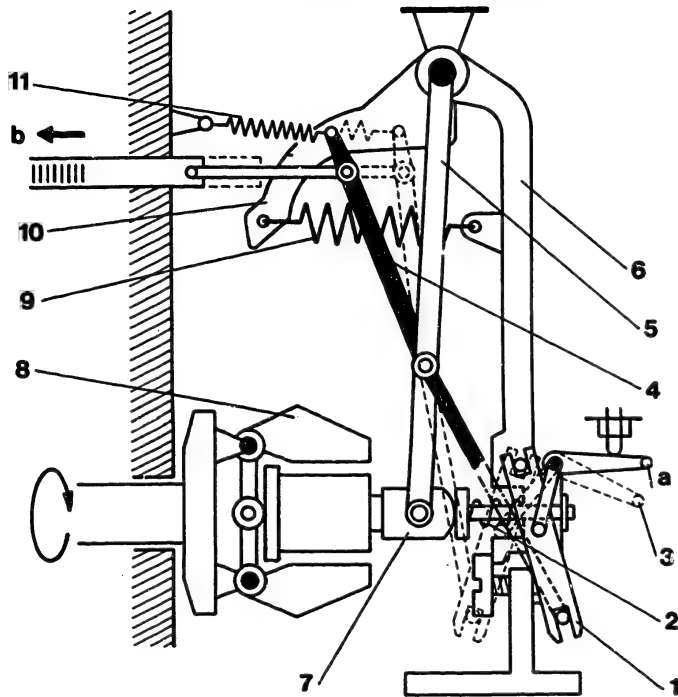
Fig. 10 Engine starting and idling control
